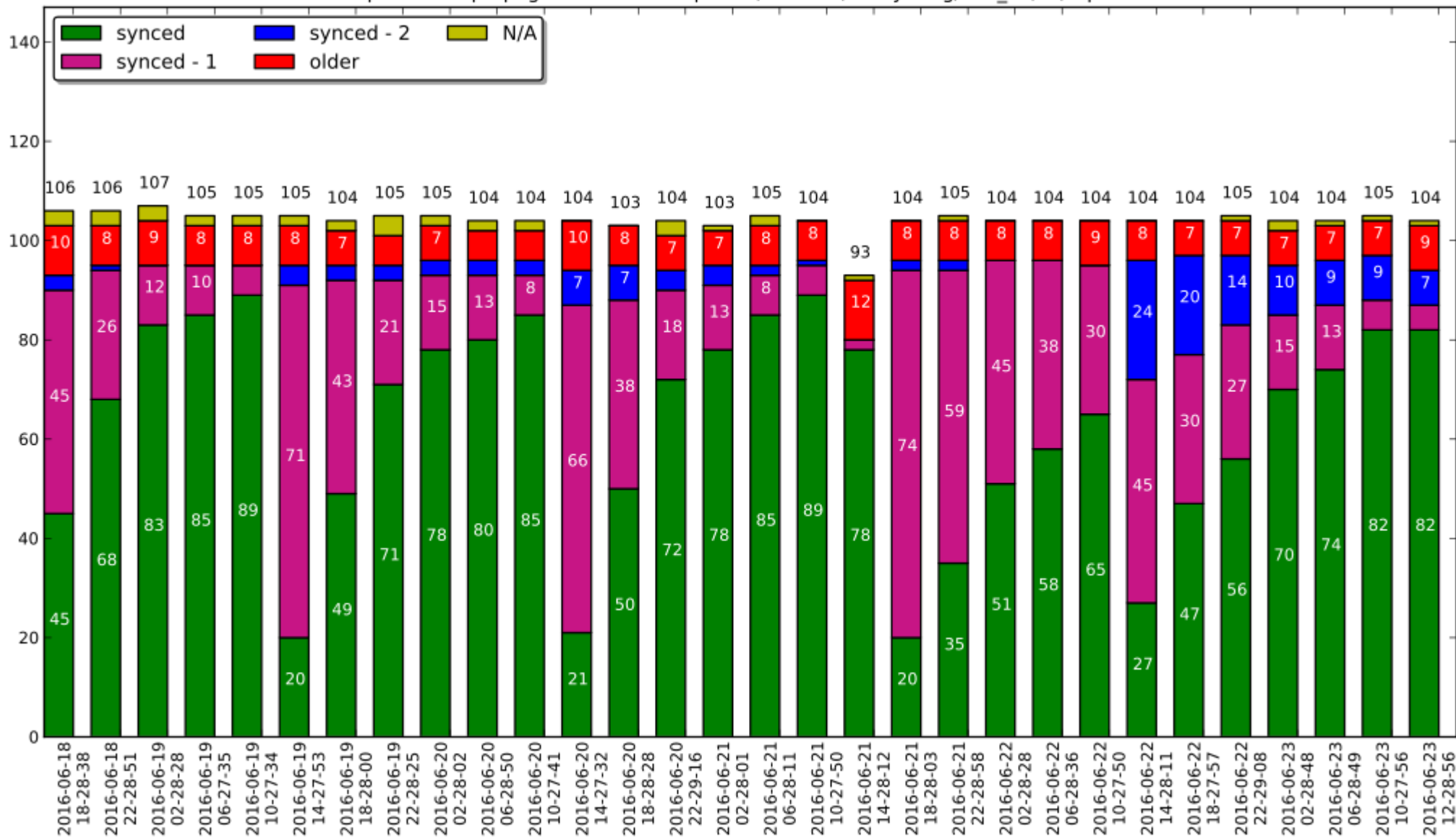
repmnd.xml propagation for development/rawhide/Everything/x86_64/os/repdata
